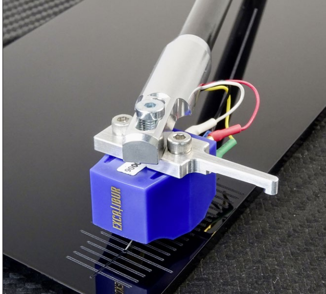
A plastic template helps with installing the cartridge. Its edges and the tonearm tube must align with the template's guide lines.
