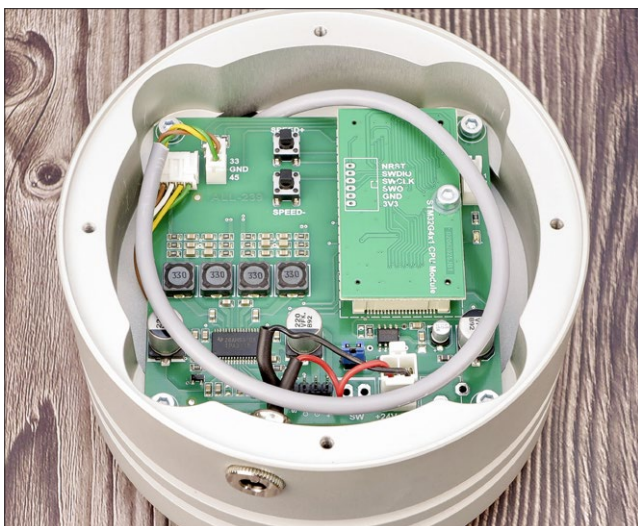
The motor control is elaborate: a microprocessor generates the sine curves for the synchronous drive and suppresses vibrations.
