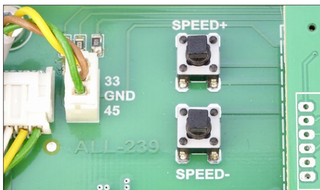
After loosening the bottom plate, the speed switches are freely accessible.
